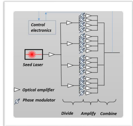
Illustration 1 CBC principle of operation
